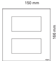
8 Module Plate Square
